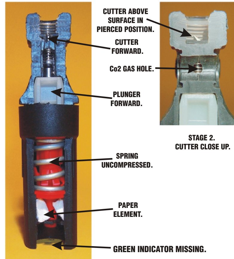
STAGE 2. FIRED UNIT.
