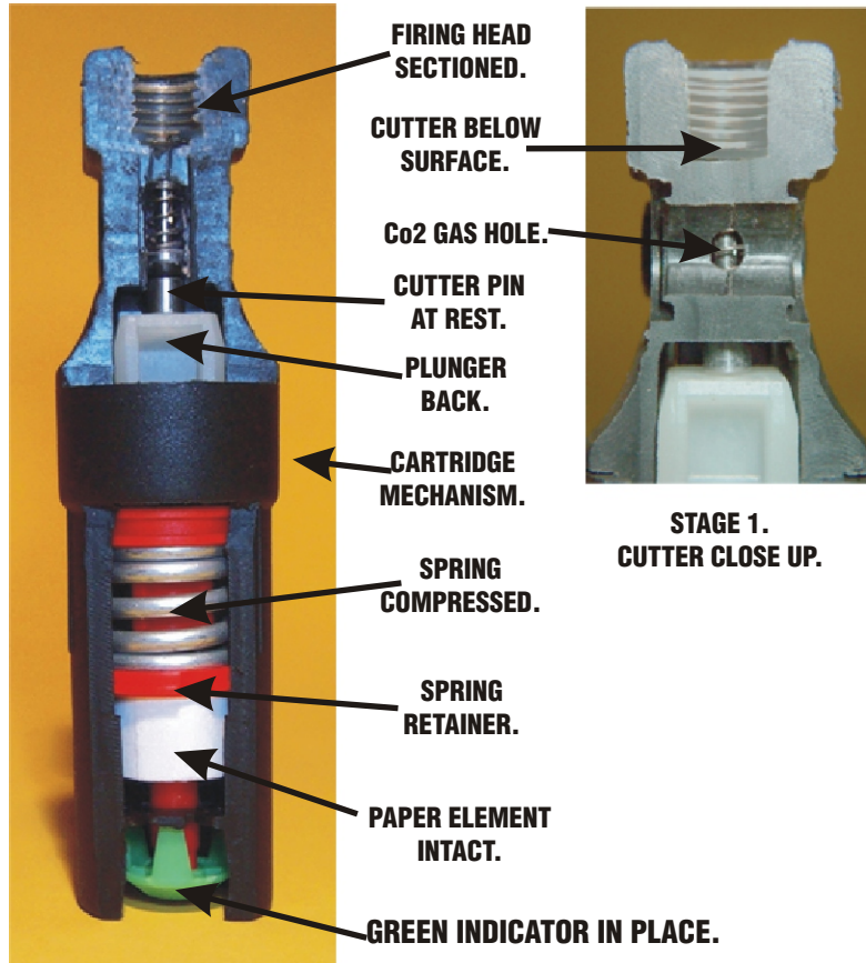
STAGE 1. UNFIRED UNIT.
